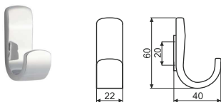
WP33 WP33-G0004 ZnAl
